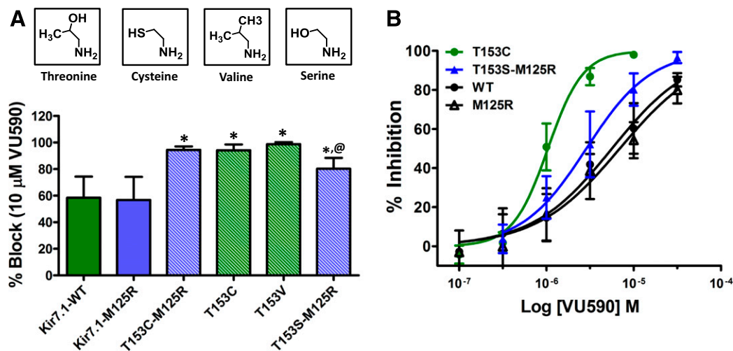
Fig. 4. Effect of mutations at position 153 on the sensitivity of Kir7.1 to VU590. (A) Mean ± S.D. percent inhibition of Kir7.1-WT (solid green bar), Kir7.1-M125R (solid blue bar) channels and mutants (striped bars) by 10 μM VU590. (B) VU590 CRC comparison of Kir7.1-WT, Kir7.1-M125R, T153C, and T153S mutants. * P < 0.05 , statistically significantly different from the respective control background (Kir7.1-WT or Kir7.1-M125R). Data were analyzed using one-way ANOVA with Bonferroni's multiple comparison test. @ P < 0.05 , statistically significantly different from T153C and T153S mutants, n \geq 5 .
