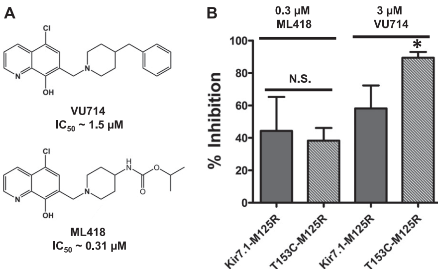
Fig. 6. T153C increases block by another low-affinity blocker, VU714. (A) Chemical structures of VU714 and ML418; (B) Mean \pm S.D. percent inhibition by 0.3 \mu\text{M} ML418 or 3 \mu\text{M} VU714 of M125R-T153C mutant. Data were analyzed using unpaired t test. * P < 0.05 statistically significantly different from the respective control background (Kir7.1-M125R), n \geq 5 . N.S., non-significant.
