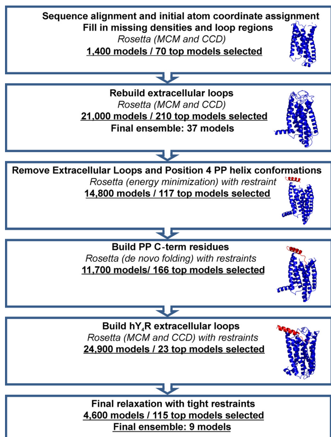
FIGURE 1. hY 4 R comparative model and PP docking work flow. An ensemble of hY 4 R comparative models was constructed through several rounds of loop building and energy minimization followed by selection of the best models. Alongside the flowchart are representative models to illustrate the evolution of the comparative model. hPP was docked through the placement of the PP helix, de novo addition of the C-terminal residues, and finally the addition of the ECLs of hY 4 R. Those steps were guided by experimentally derived restraints and followed by selection of the top models.
