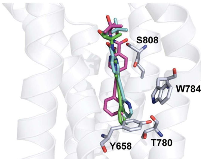
Figure 8. mGlu 5 binding pose for pure-PAMs 31i (cyan color) and 38t (green color) and ago-PAM 19 (magenta).
